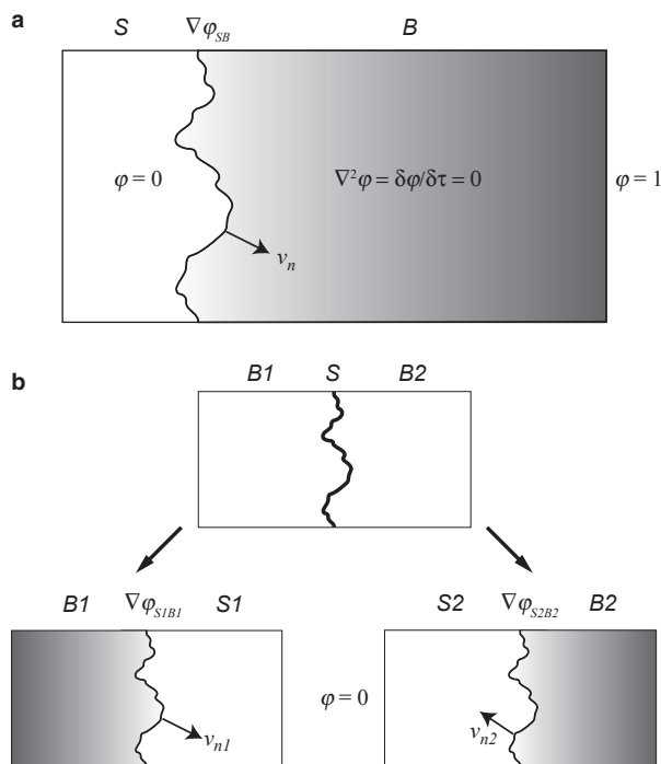
Fig. 2 Laplacian models of interface growth. (a) Unidirectional model. Phase S grows with velocity v_n as a function of gradient \nabla \varphi_{SB} at the S – B interface. Field distribution of \varphi within B obeys the Laplace equation; \varphi within S is zero. (b) Bidirectional model of bone growth at suture interface. The system is subdivided into complementary subsystems [ S1 , B1 ] and [ S2 , B2 ]. Bone deposition/resorption rates are evaluated as functions of strain gradients ( \nabla \varphi_{S1B1} and \nabla \varphi_{S2B2} ) on opposite sides of the suture line.
